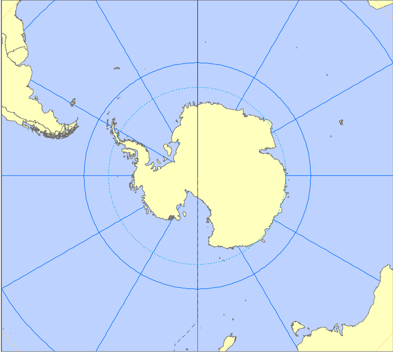
Azimuthal Equidistant Projection
